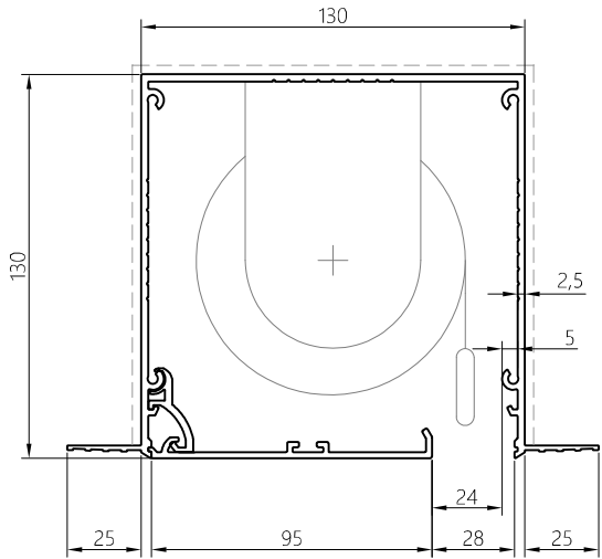
SIDE BOX S130x50SS (OPTIONAL)
