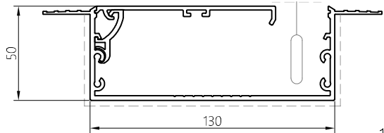
HEM BAR BOX S130x50SS (OPTIONAL)
